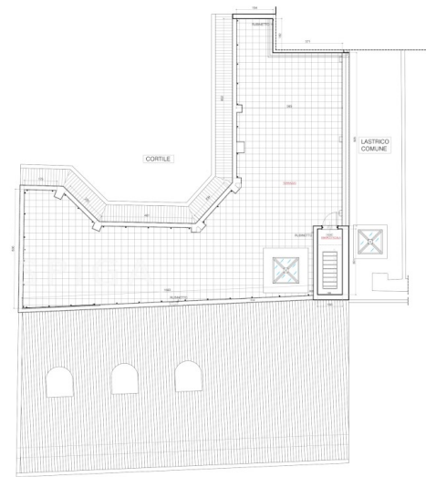
PLANIMETRIA 5° PIANO
